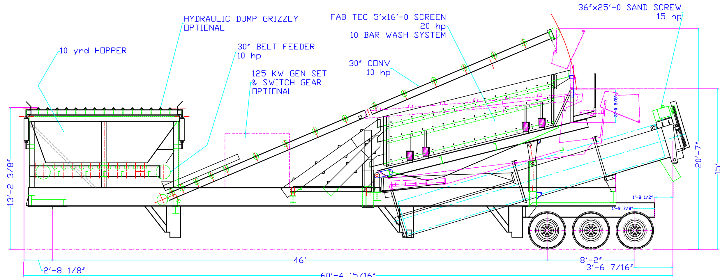
WASH PLANT with FEEDER
